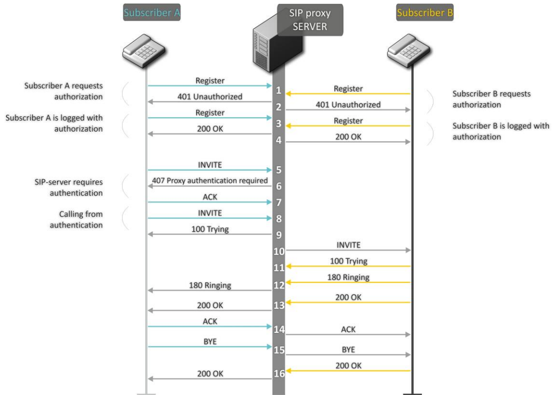
Fig. 15 — Call algorithm involving SIP proxy server
