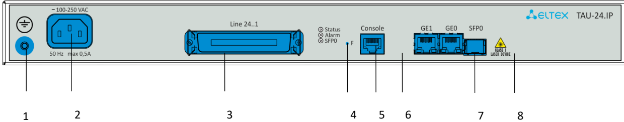
Figure 4a – TAU-24.IP AC front panel appearance
