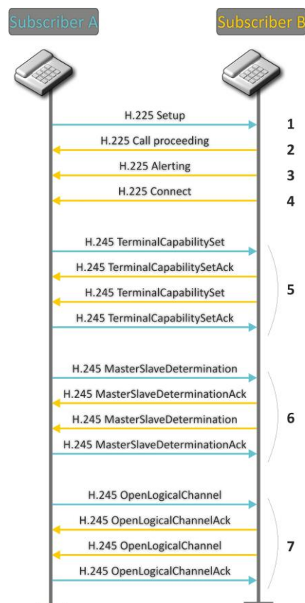
Fig. 17 — H.323 call algorithm
