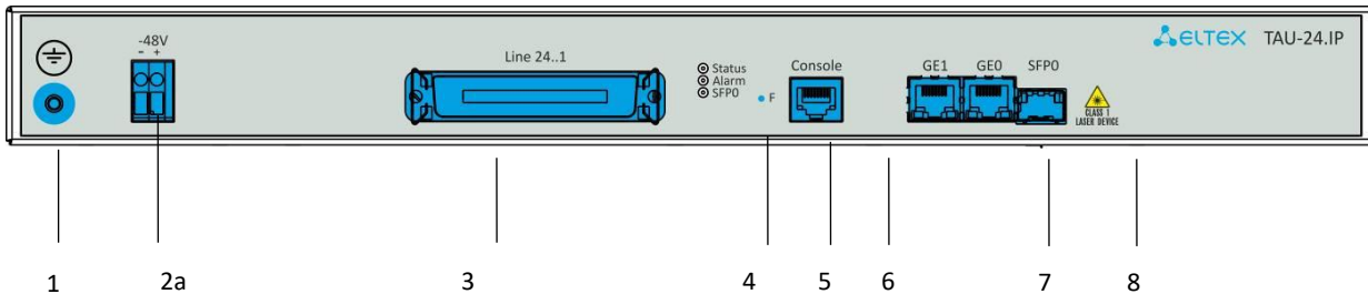
Figure 4c – TAU-24.IP DC front panel
