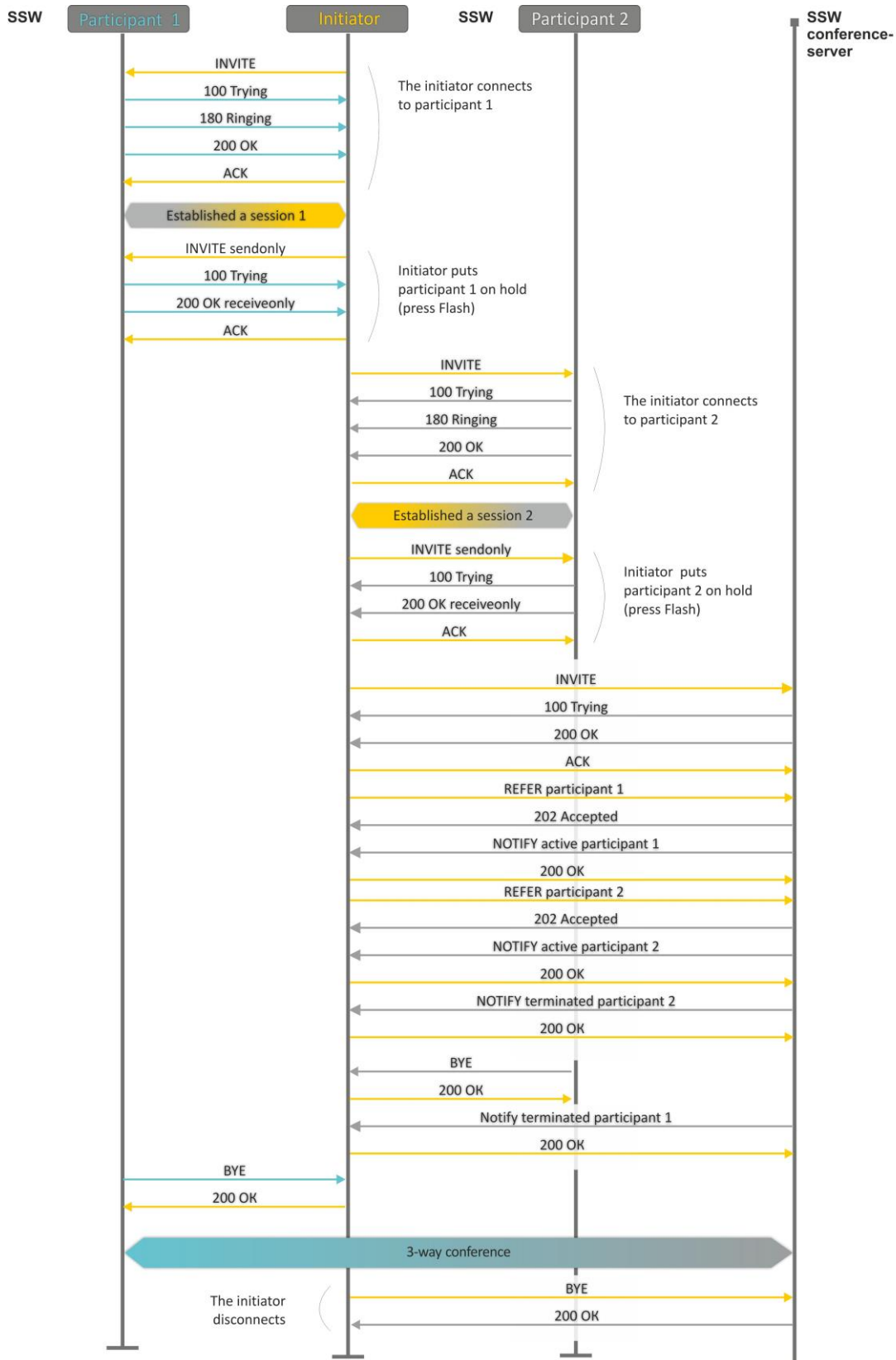
Fig. 12 — Algorithm of '3-way conference' service performed at the conference server via SIP protocol (REFER to focus)
