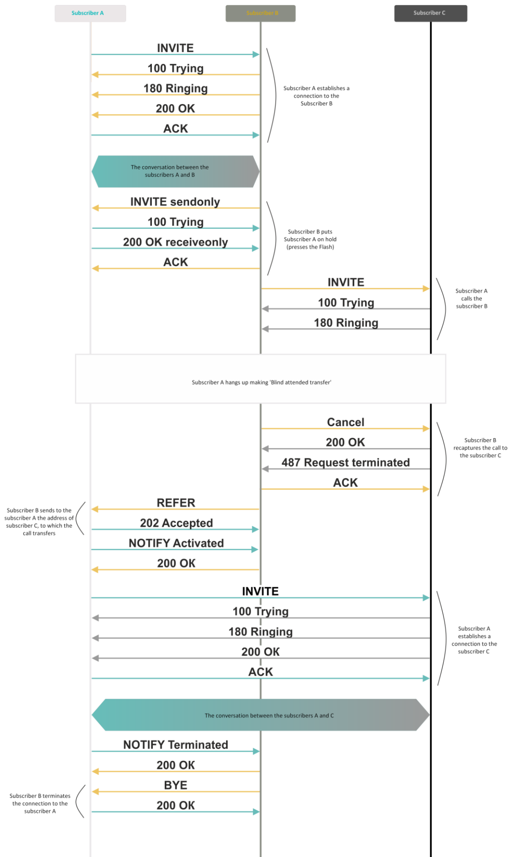
Fig. 10 — Algorithm of "Blind attended transfer" service by Subscriber B via SIP protocol
