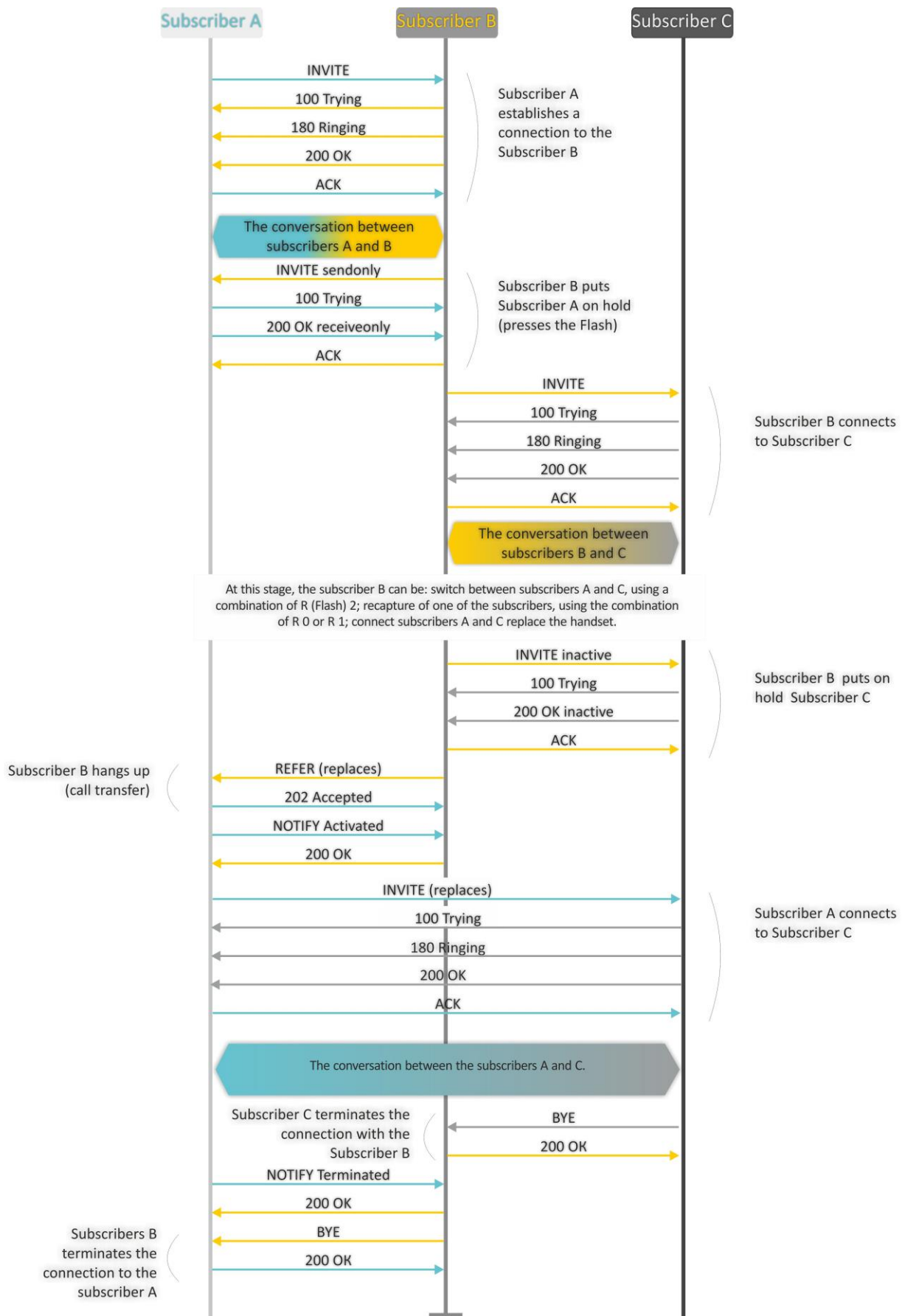
Fig. 8 — Algorithm of 'Attended call transfer' service performed by Subscriber B via SIP protocol
