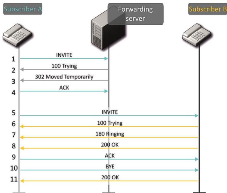
Fig. 16 — Call algorithm involving forwarding server
