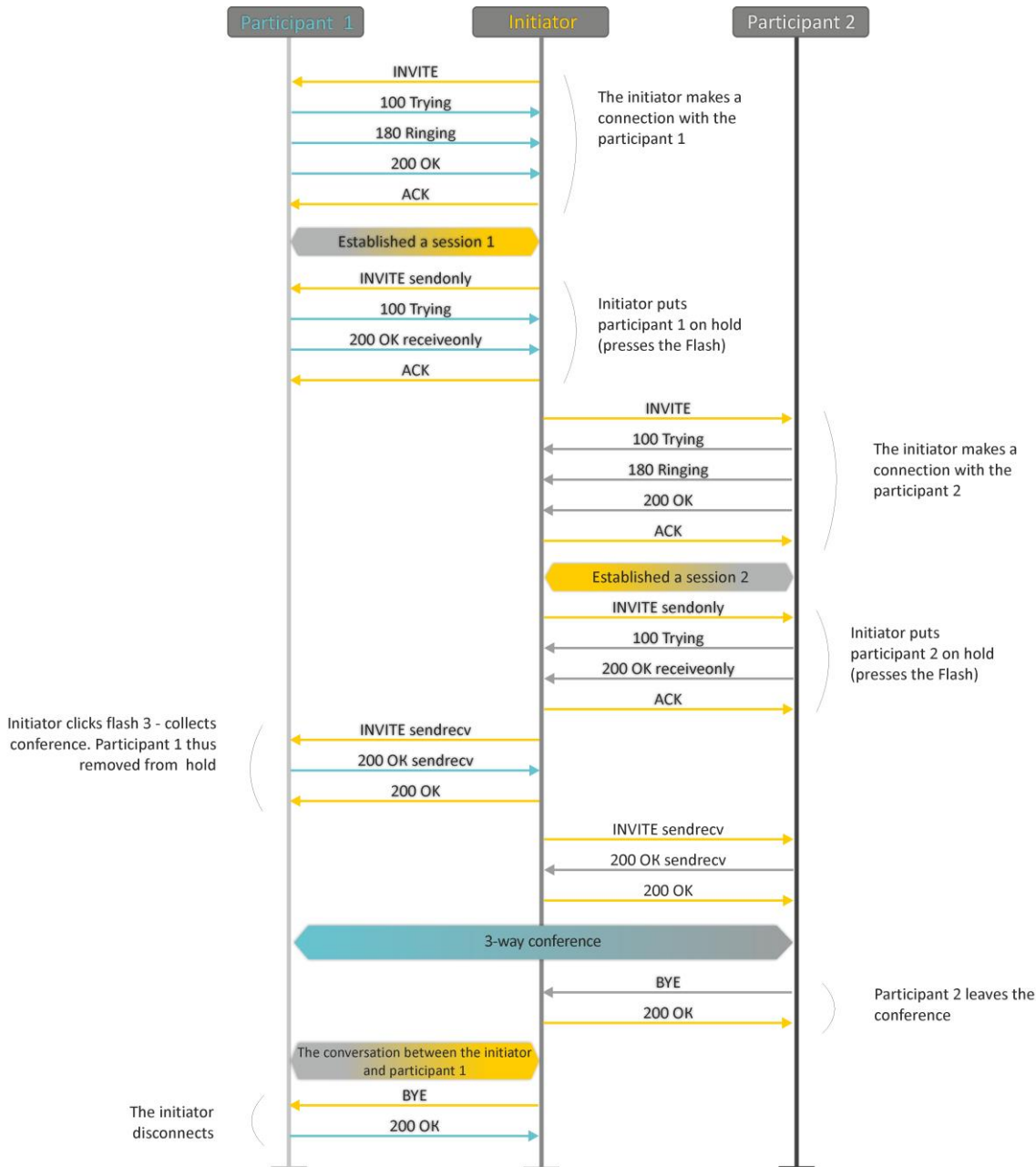
Fig. 11 — Algorithm of '3-way conference' service performed locally on the device via SIP protocol
