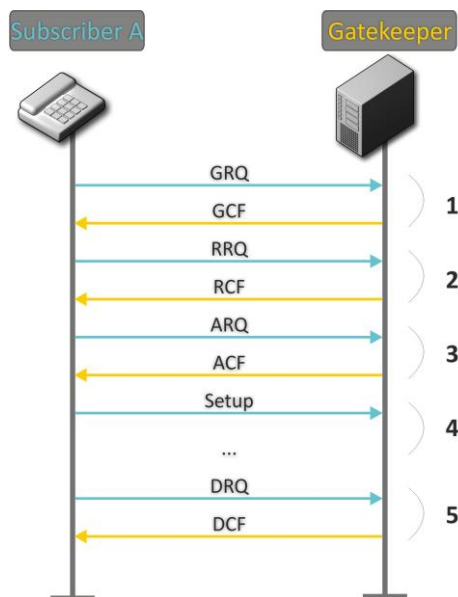
Fig. 18 — Gatekeeper call algorithm
