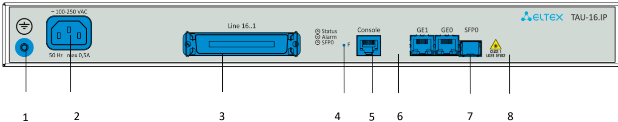
Figure 4b – TAU16.IP AC front panel appearance
