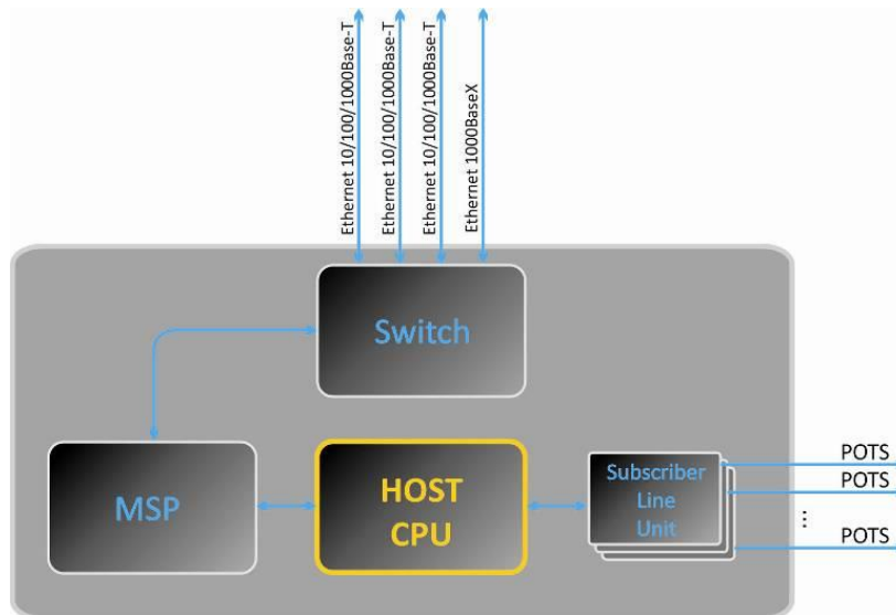
Fig. 3 - TAU-24/16.IP functional diagram
