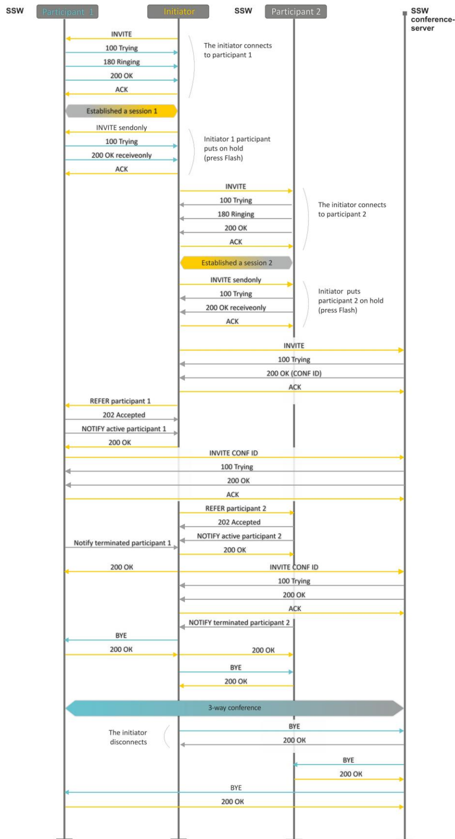
Fig. 13 — Algorithm of '3-way conference' service performed at the conference server via SIP protocol (REFER to user)
